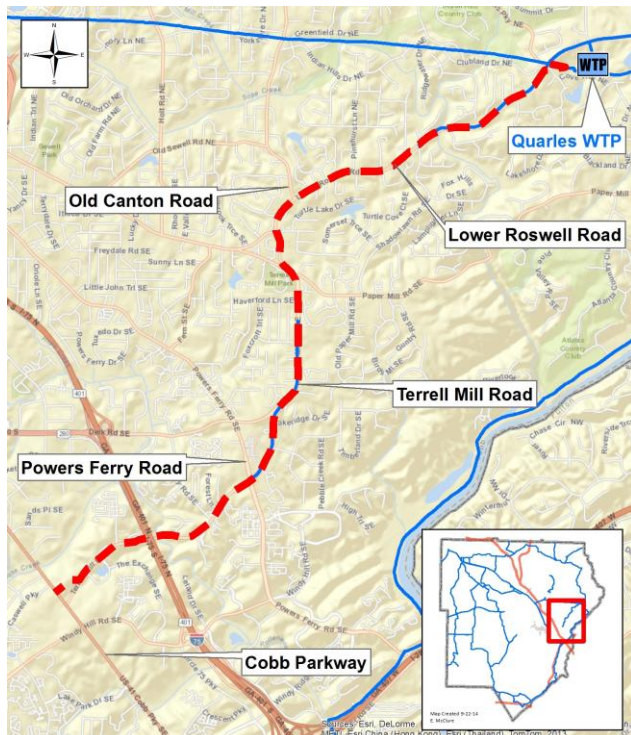
Planned Water Main Route
